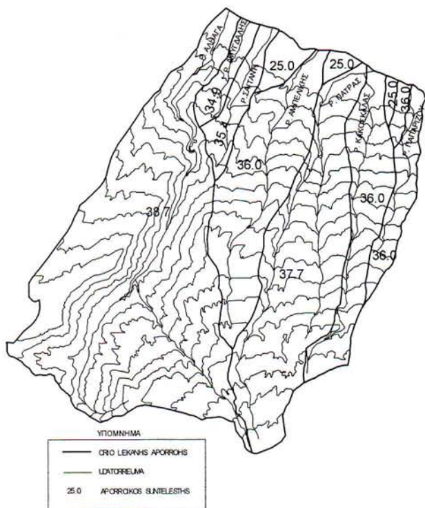
Figure 4: Map of composite runoff curve numbers CN_c per watershed, scale 1:82000
